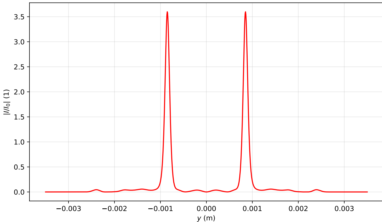
Intensity profile I(x=0, y, z=2.468)/I_0 , P_{in}=20.0\text{Pcr} , artificial time
