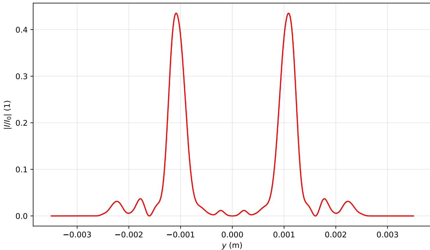
Intensity profile I(x=0, y, z=3.025)/I_0 , P_{in}=20.0P_{cr} , artificial time
