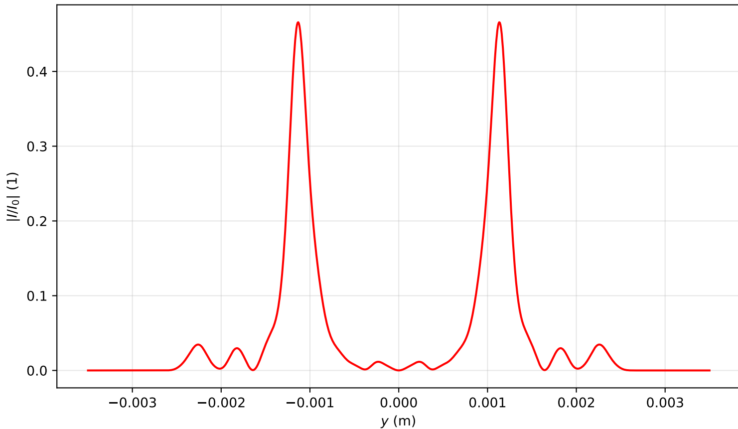
Intensity profile I(x=0, y, z=3.105)/I_0 , P_{in}=20.0\text{Pcr} , artificial time
