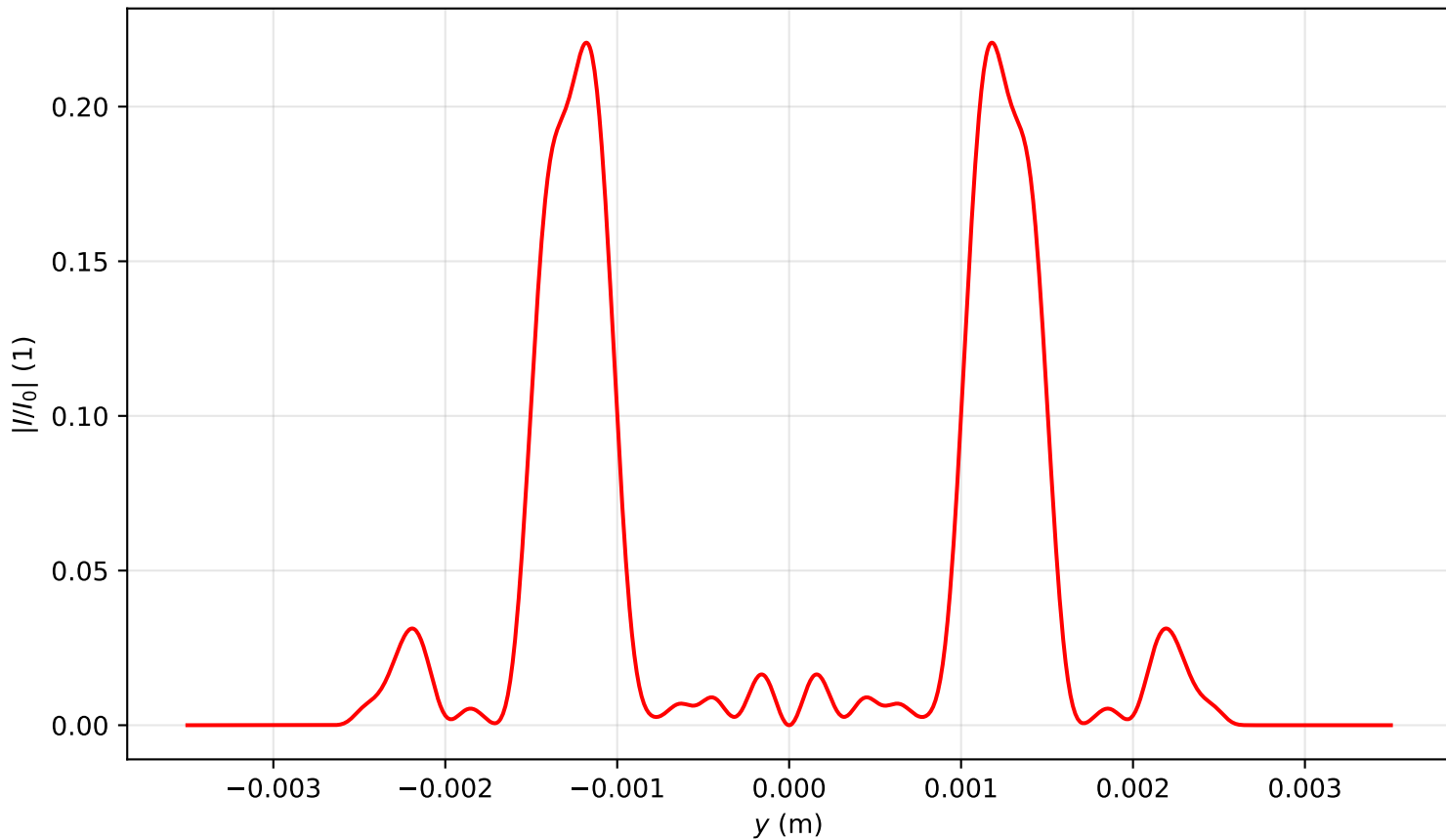
Intensity profile I(x=0, y, z=3.344)/I_0 , P_{in}=20.0\text{Pcr} , artificial time
