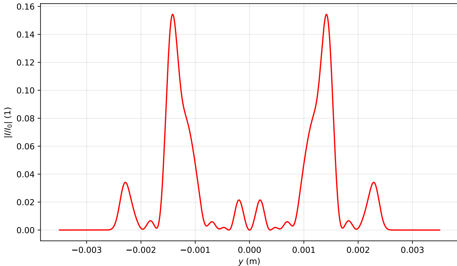
Intensity profile I(x = 0, y, z = 3.503)/I_0 , P_{in}=20.0\text{Pcr} , artificial time
