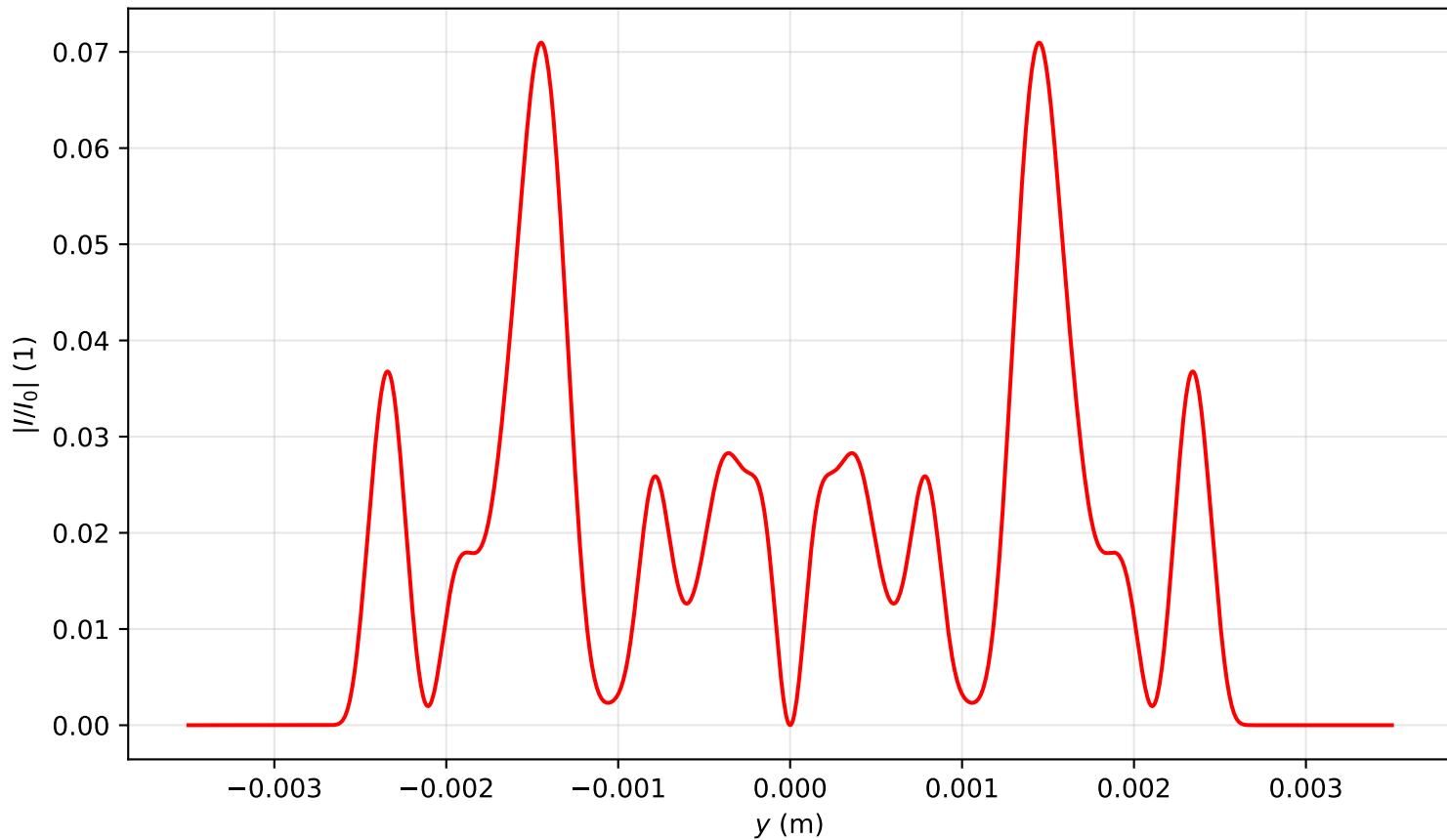
Intensity profile I(x=0, y, z=3.821)/I_0 , P_{in}=20.0\text{Pcr} , artificial time
