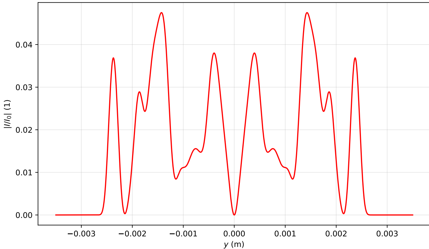
Intensity profile I(x=0, y, z=3.901)/I_0 , P_{in}=20.0\text{Pcr} , artificial time
