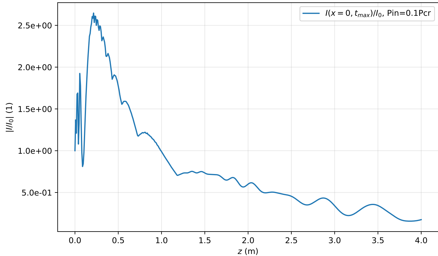
I(x=0, t_{max}, z)/I_0 , Pin=0.1Pcr
