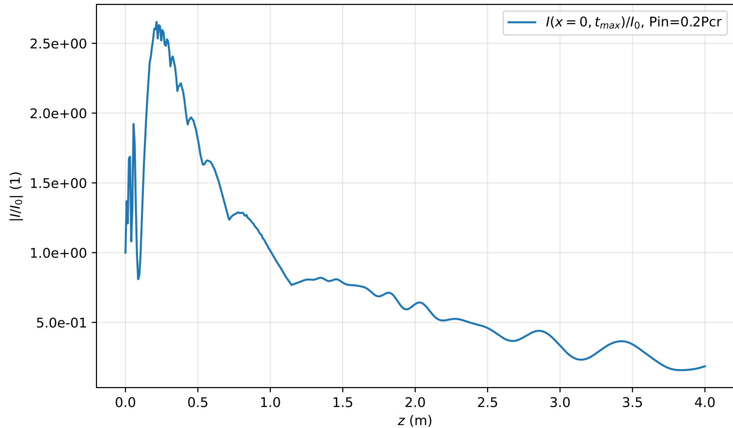
I(x=0, t_{max}, z)/I_0 , Pin=0.2Pcr
