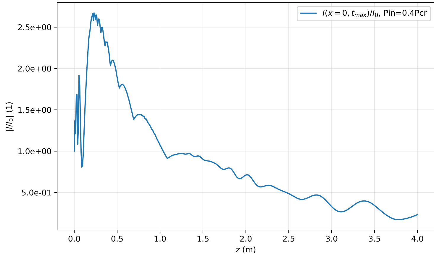
I(x=0, t_{max}, z)/I_0 , Pin=0.4Pcr
