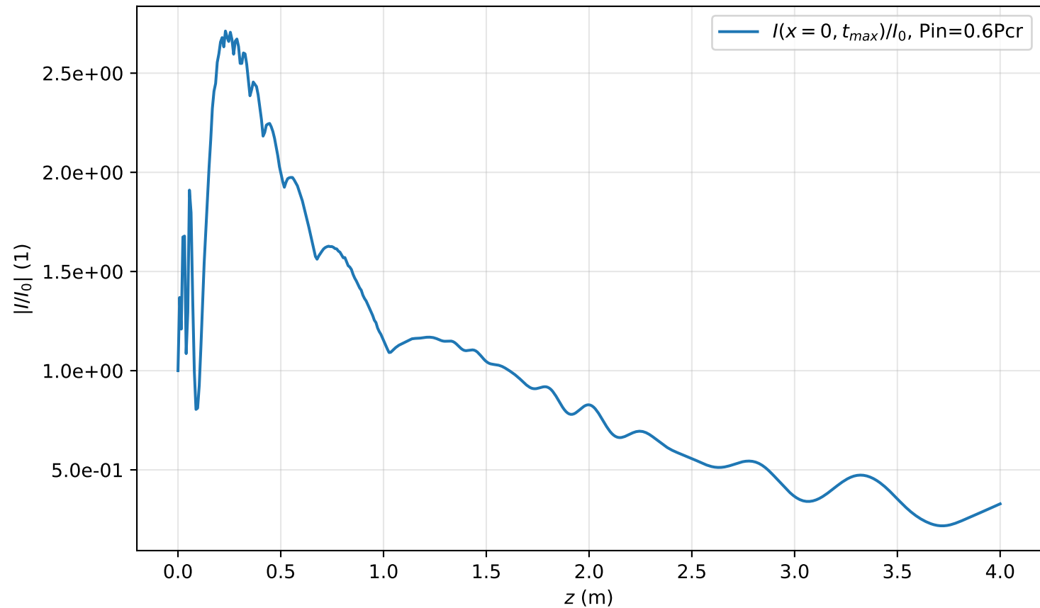
I(x=0, t_{max}, z)/I_0 , Pin=0.6Pcr
