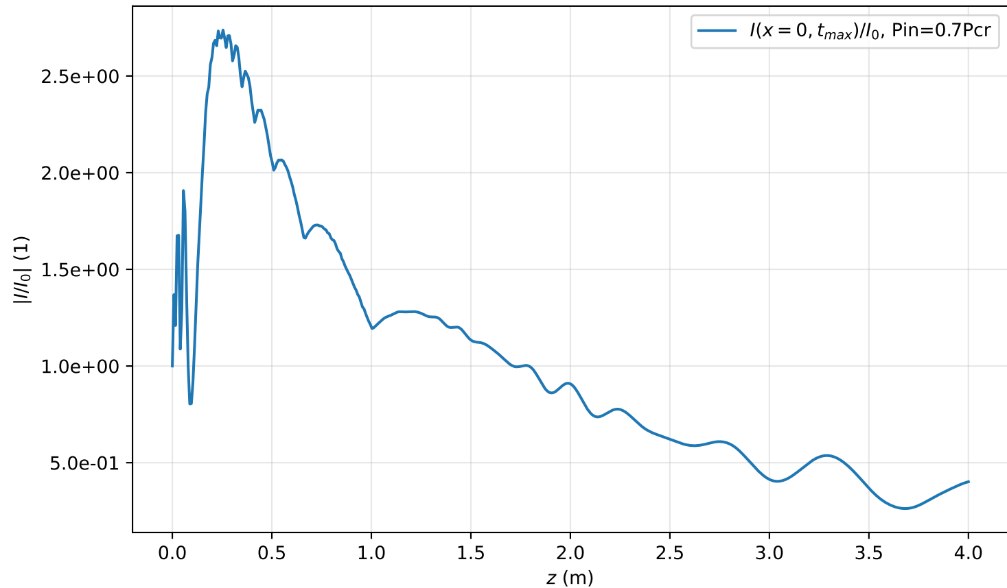
I(x=0, t_{max}, z)/I_0 , \text{Pin}=0.7\text{Pcr}
