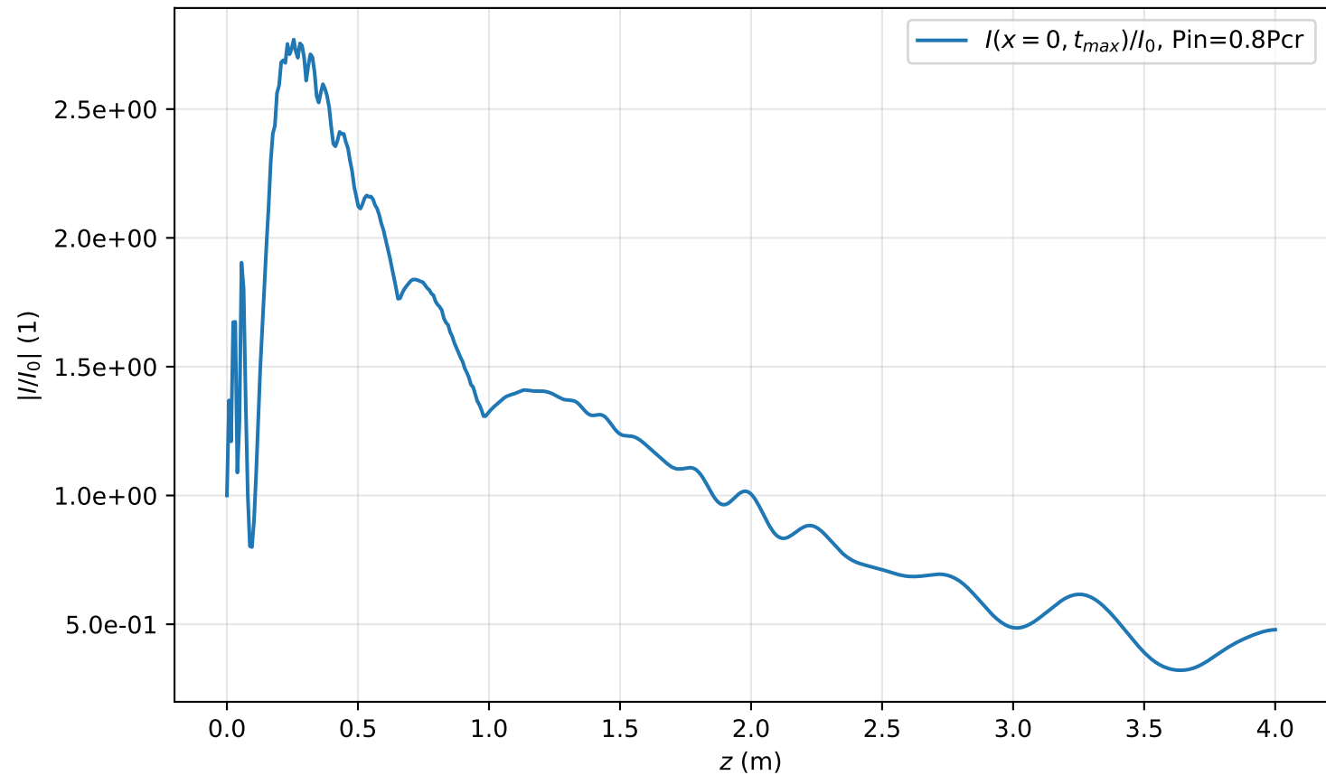
I(x=0, t_{max}, z)/I_0 , Pin=0.8Pcr
