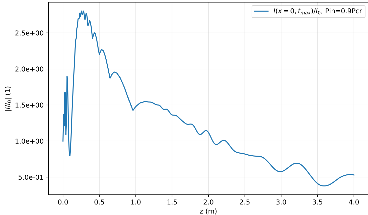
I(x=0, t_{max}, z)/I_0 , Pin=0.9Pcr
