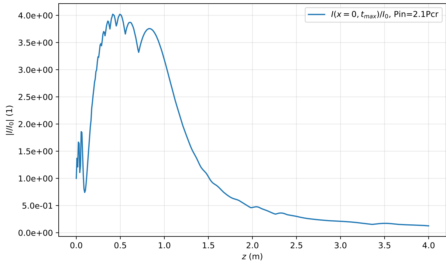
I(x=0, t_{max}, z)/I_0 , Pin=2.1Pcr
