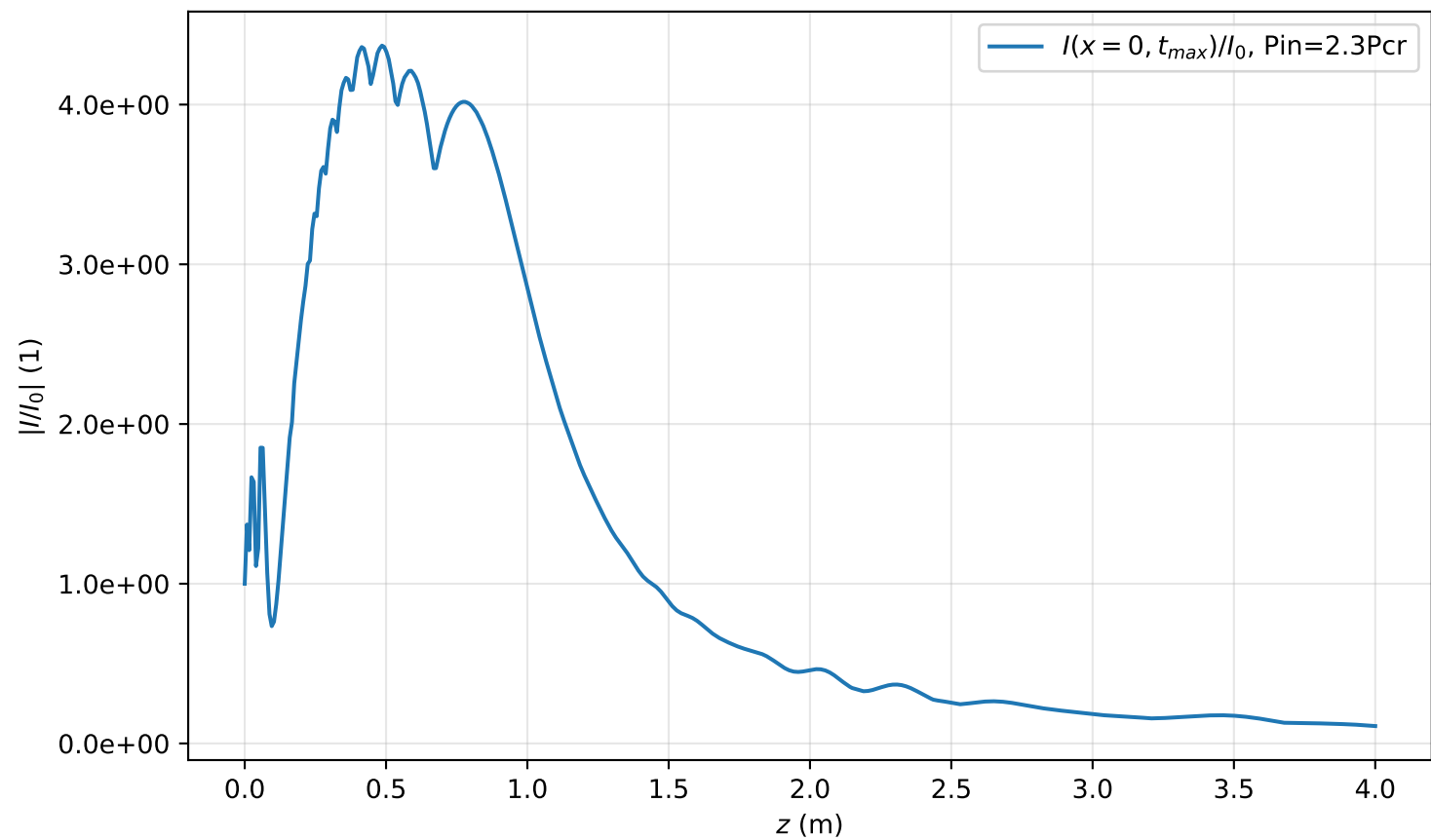
I(x=0, t_{max}, z)/I_0 , Pin=2.3Pcr
