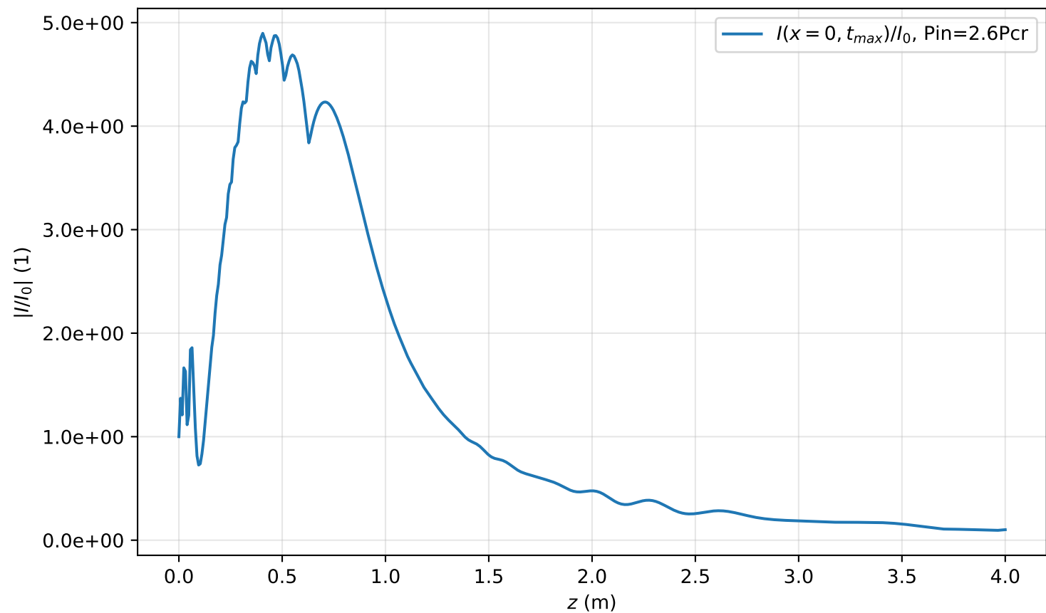
I(x=0, t_{max}, z)/I_0 , Pin=2.6Pcr
