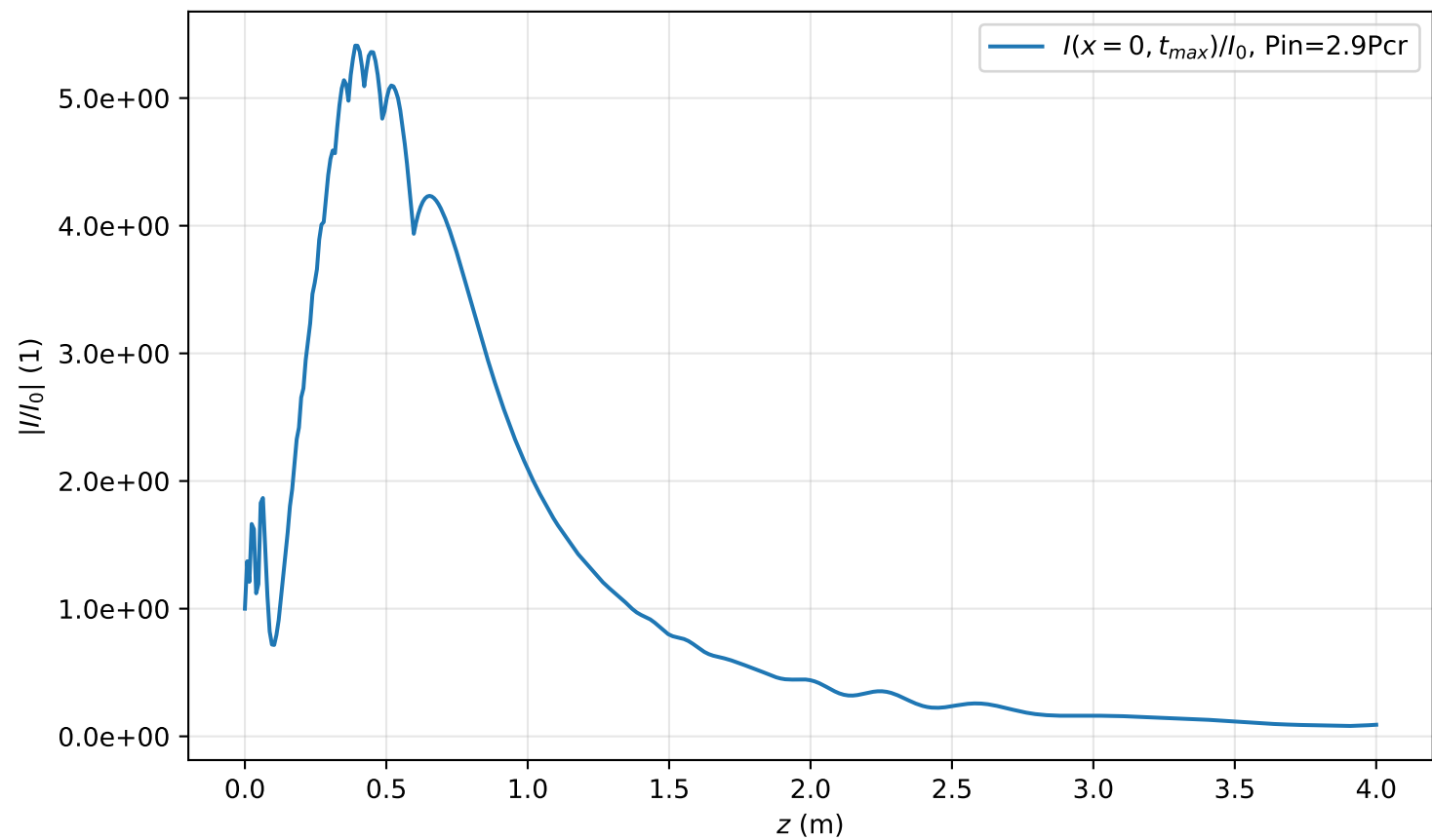
I(x=0, t_{max}, z)/I_0 , Pin=2.9Pcr
