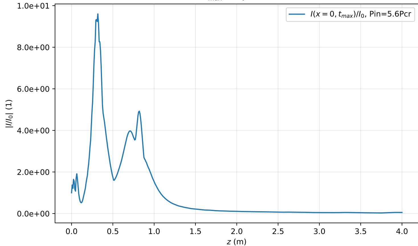
I(x=0, t_{max}, z)/I_0 , Pin=5.6Pcr
