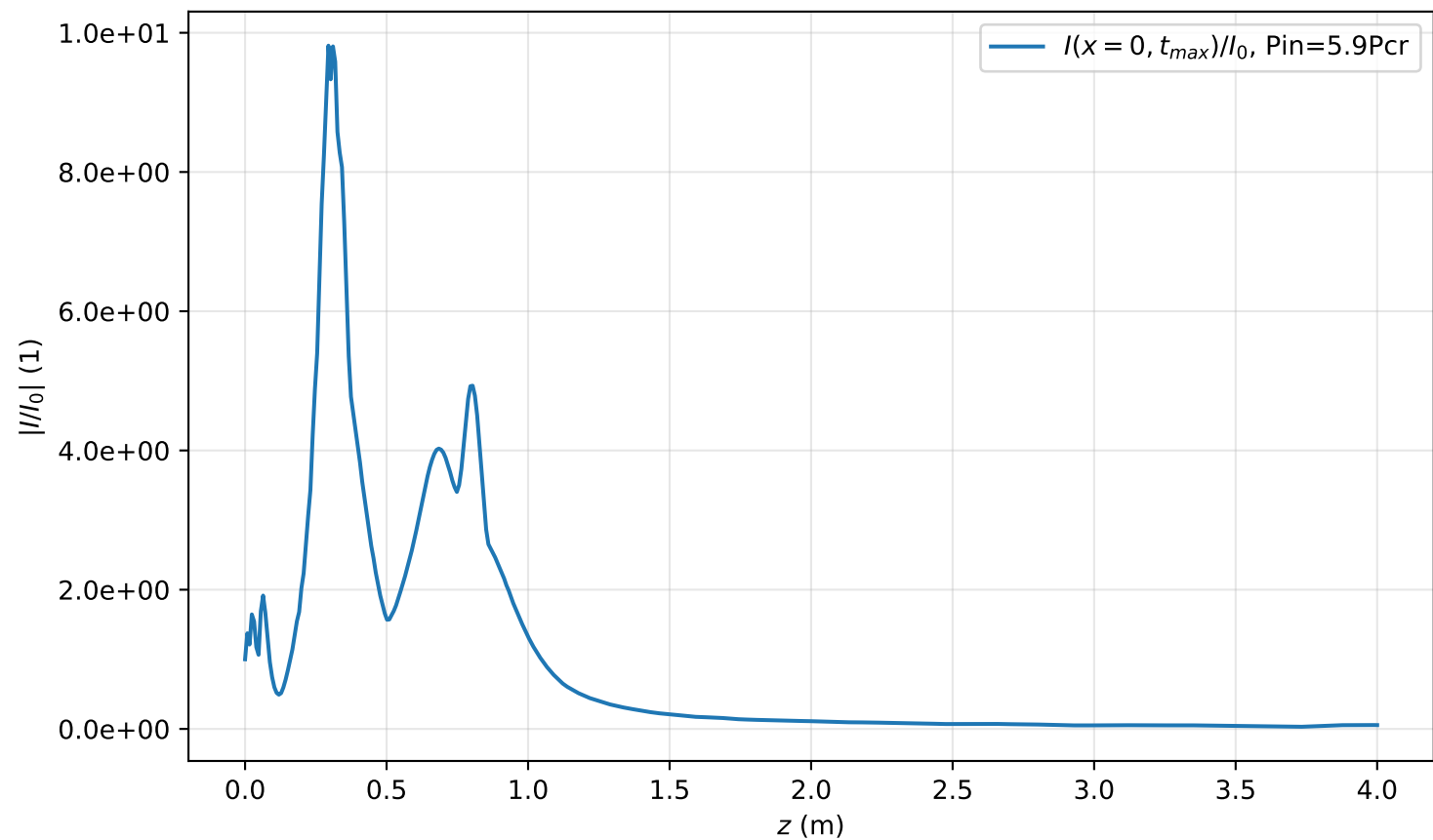
I(x=0, t_{max}, z)/I_0 , Pin=5.9Pcr
