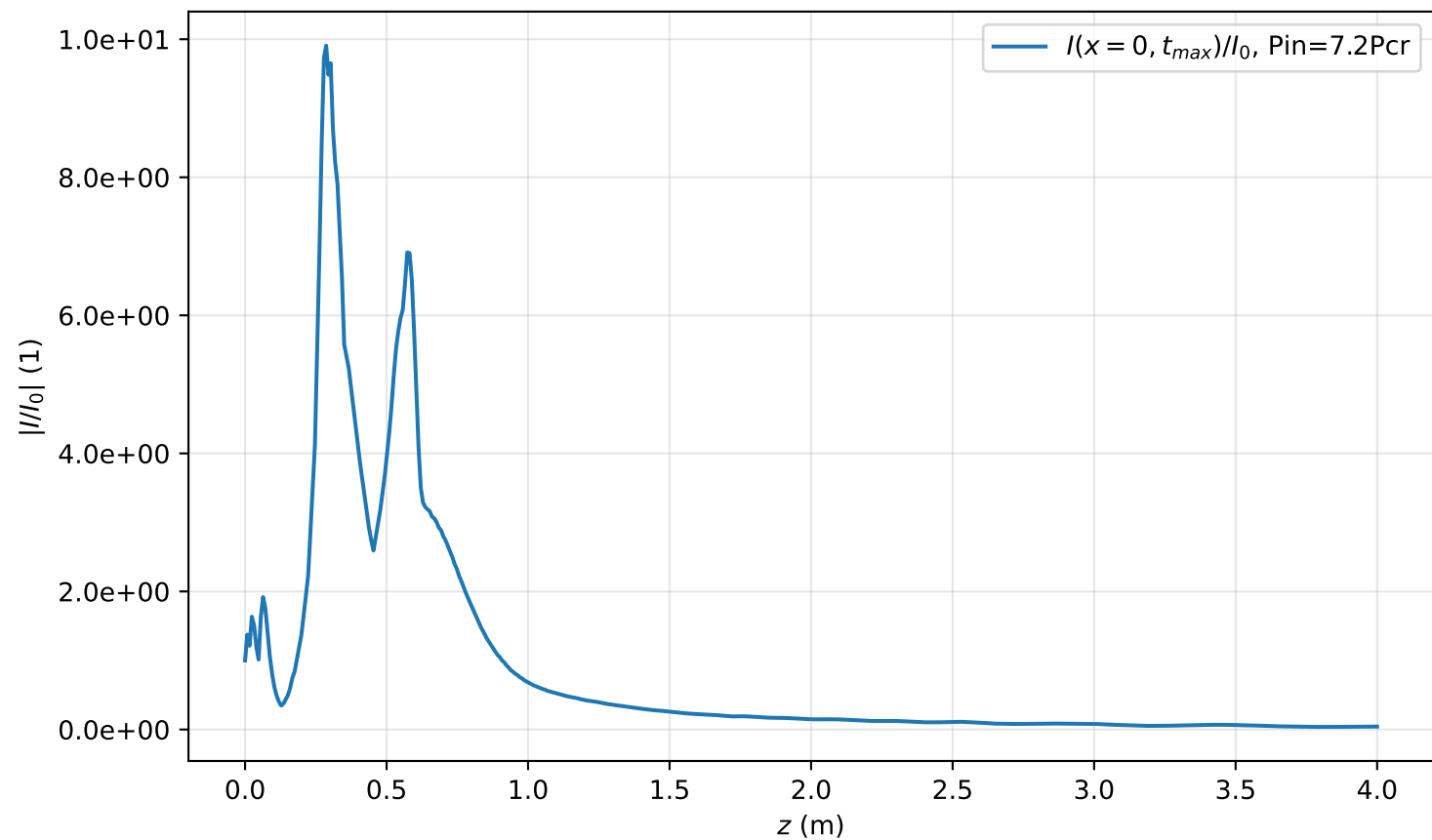
I(x=0, t_{max}, z)/I_0 , Pin=7.2Pcr
