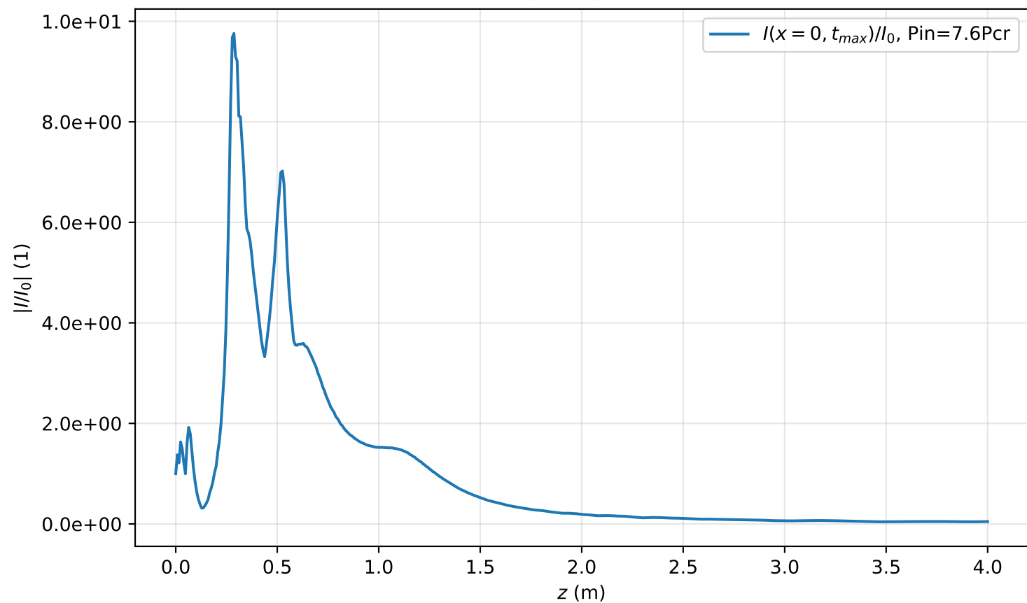
I(x=0, t_{max}, z)/I_0 , Pin=7.6Pcr
