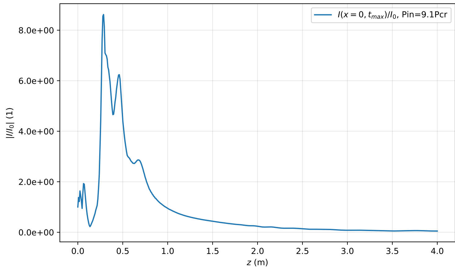
I(x=0, t_{max}, z)/I_0 , Pin=9.1Pcr
