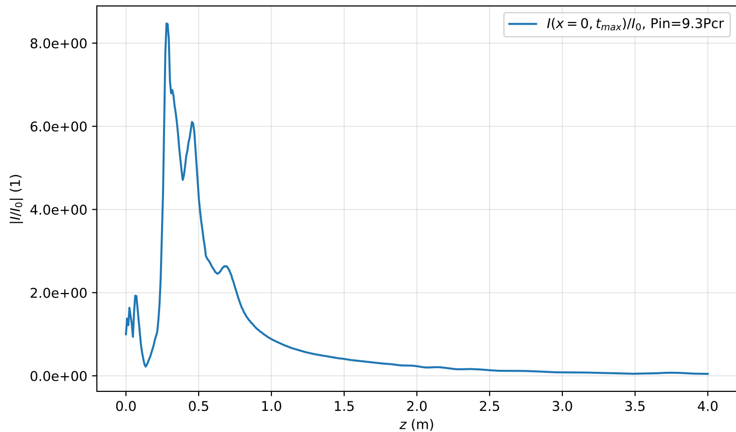
I(x=0, t_{max}, z)/I_0 , Pin=9.3Pcr
