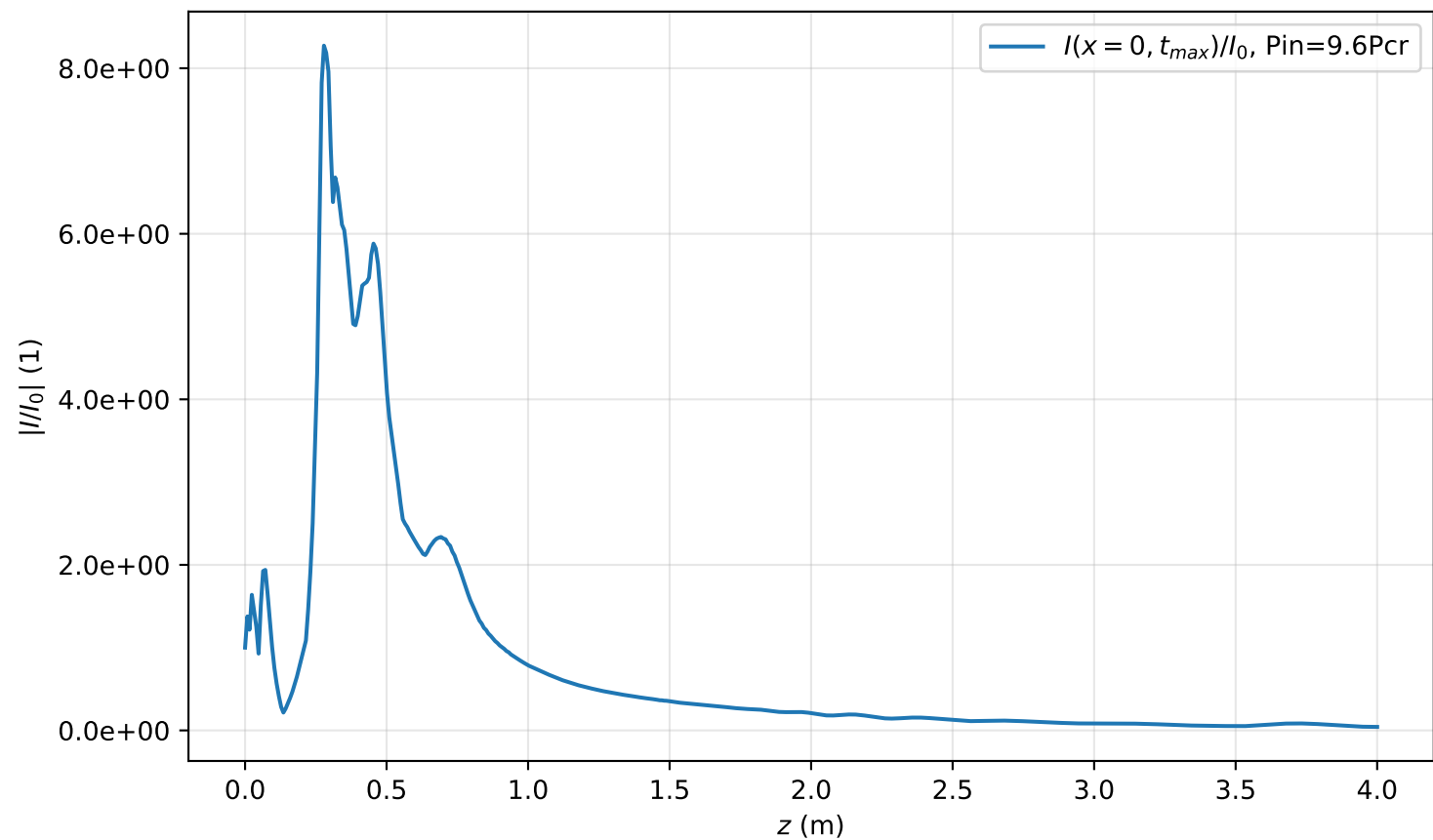
I(x=0, t_{max}, z)/I_0 , Pin=9.6Pcr
