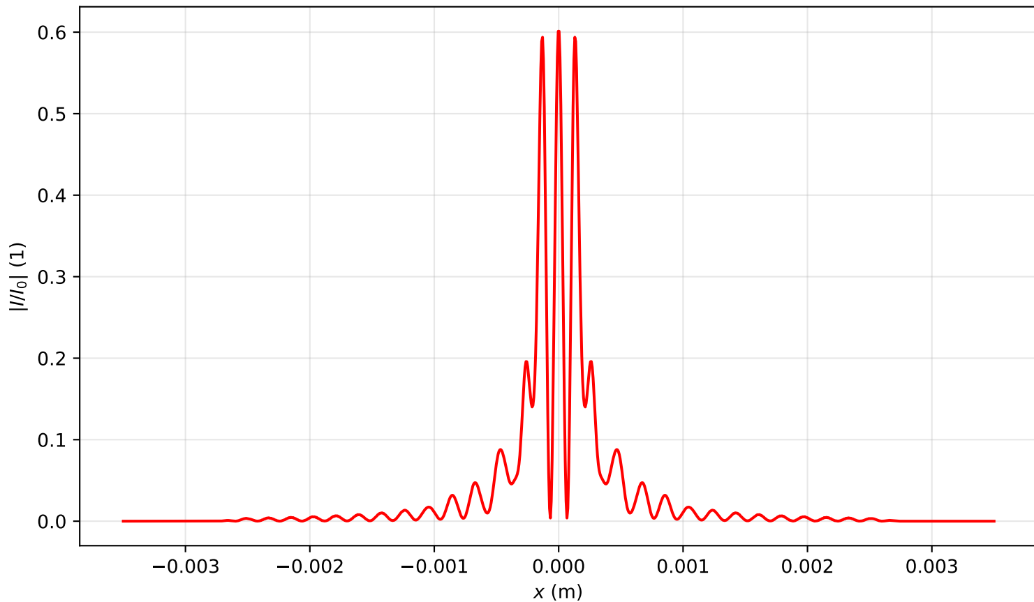
Intensity profile I(x, y = 0, z = 0.159)/I_0 , P_{in}=11.0P_{cr} , artificial time
