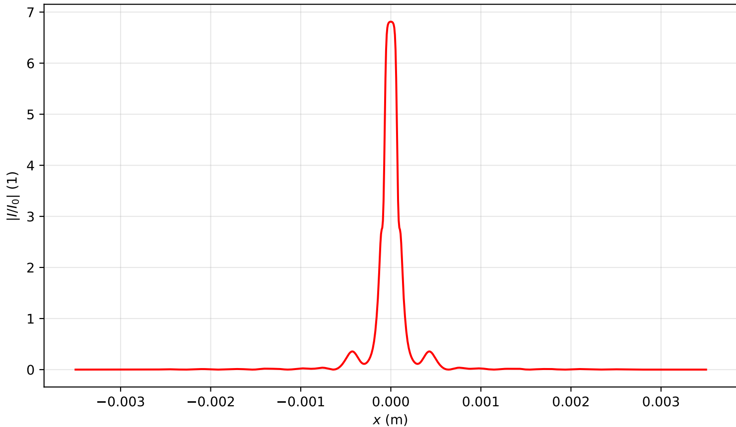
Intensity profile I(x, y = 0, z = 0.318)/I_0 , P_{in}=11.0P_{cr} , artificial time
