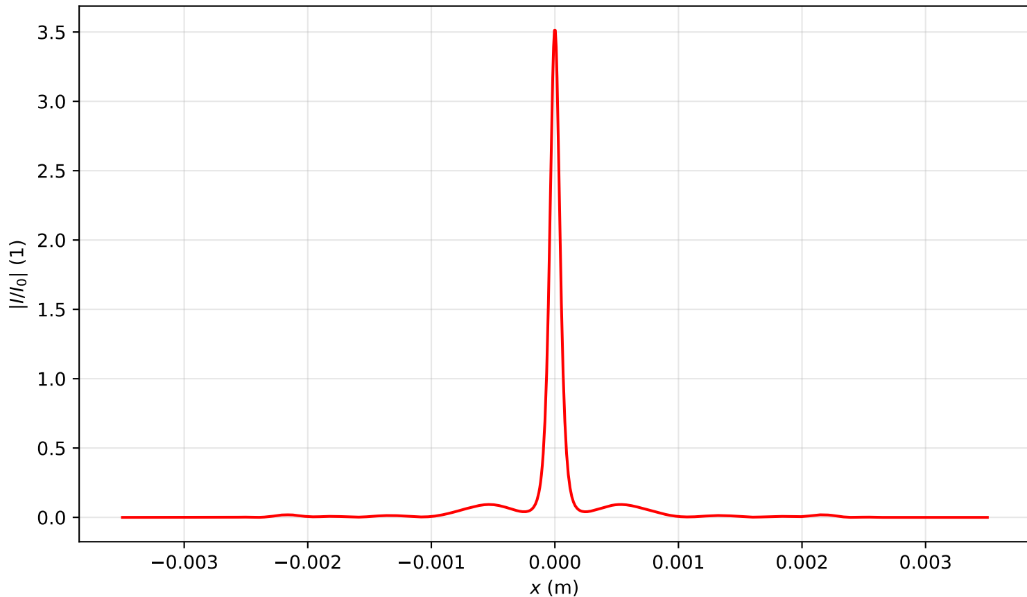
Intensity profile I(x, y = 0, z = 0.796)/I_0 , P_{in}=11.0P_{cr} , artificial time
