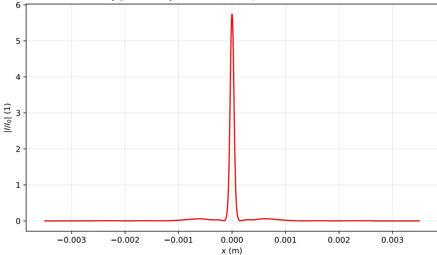
Intensity profile I(x, y = 0, z = 0.955)/I_0 , P_{in}=11.0P_{cr} , artificial time
