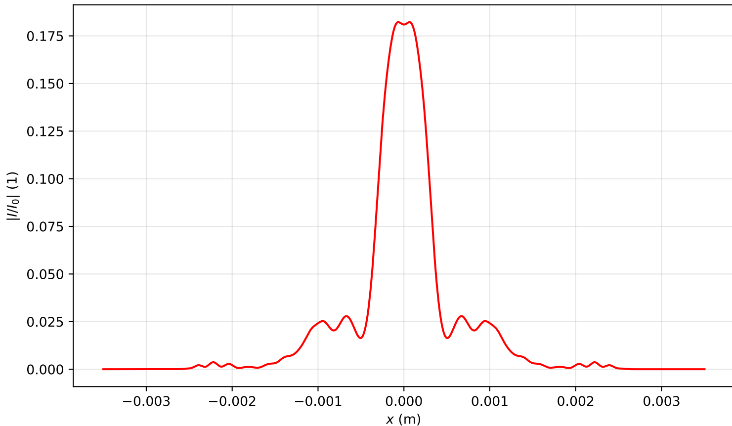
Intensity profile I(x, y = 0, z = 1.274)/I_0 , P_{in}=11.0P_{cr} , artificial time
