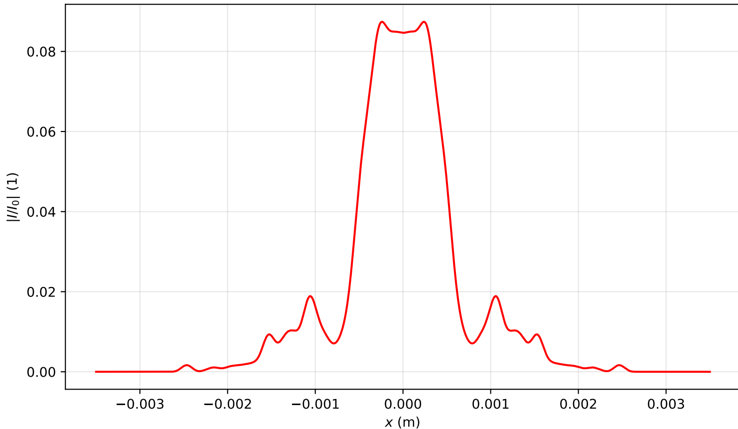
Intensity profile I(x, y = 0, z = 1.592)/I_0 , P_{in}=11.0P_{cr} , artificial time
