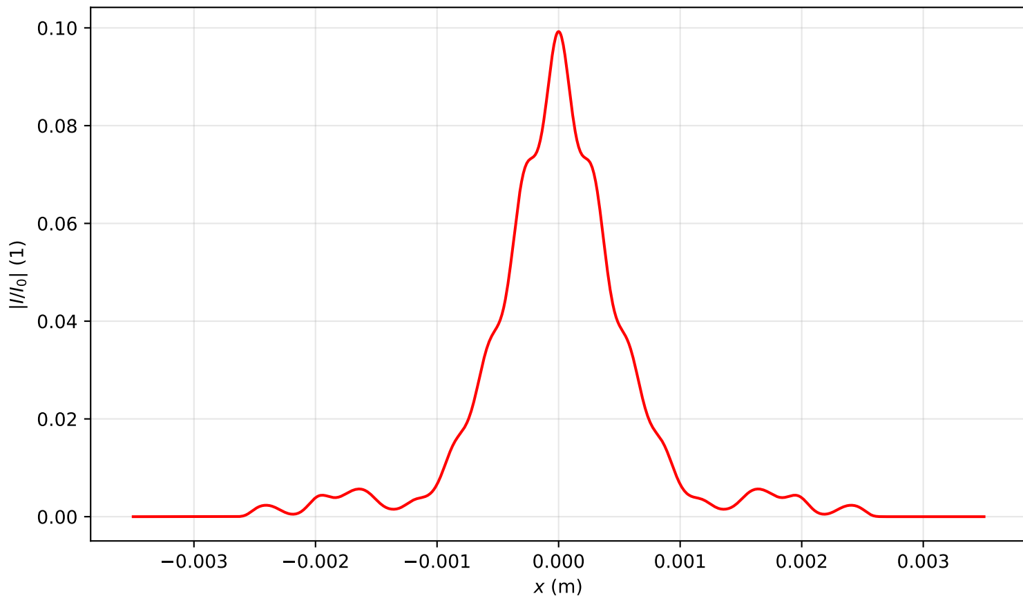
Intensity profile I(x, y = 0, z = 2.229)/I_0 , P_{in}=11.0P_{cr} , artificial time
