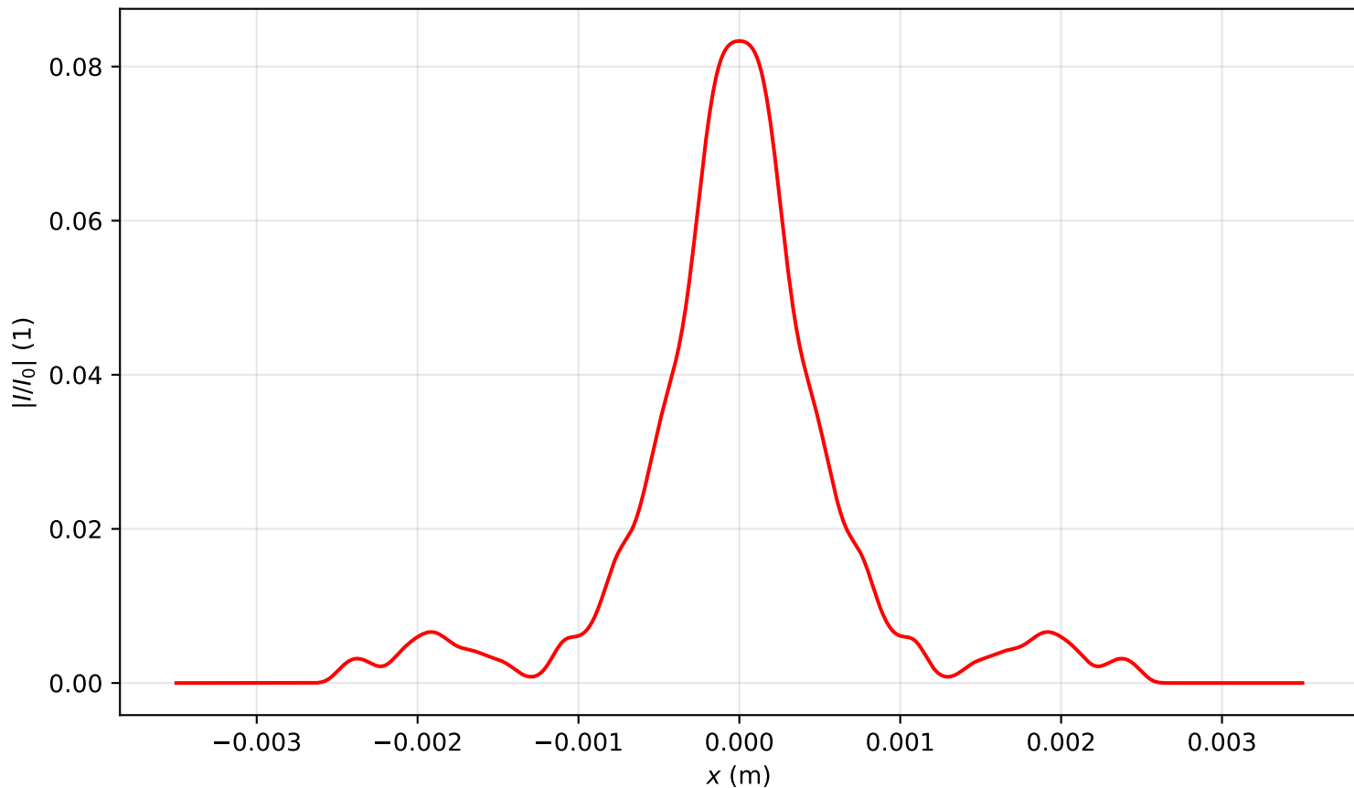
Intensity profile I(x, y = 0, z = 2.388)/I_0 , P_{in}=11.0P_{cr} , artificial time
