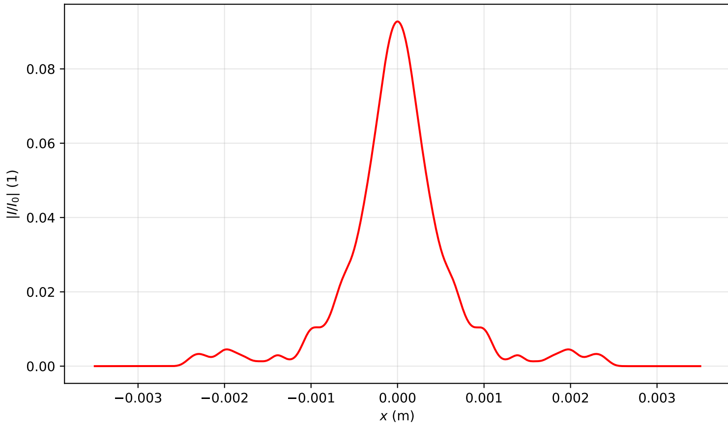
Intensity profile I(x, y = 0, z = 2.548)/I_0 , P_{in}=11.0P_{cr} , artificial time
