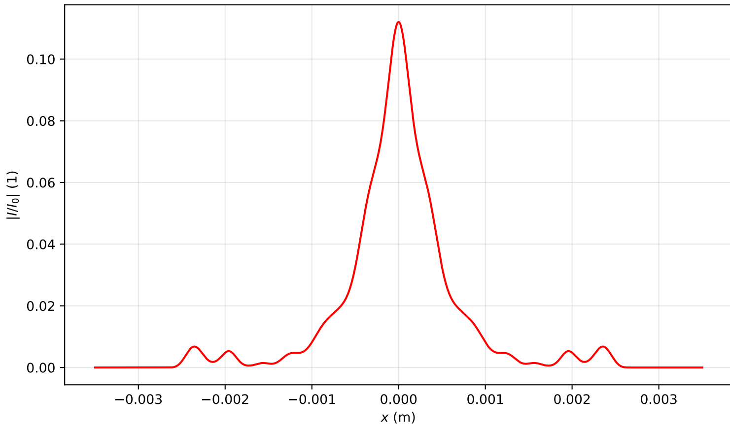
Intensity profile I(x, y = 0, z = 2.707)/I_0 , P_{in}=11.0P_{cr} , artificial time
