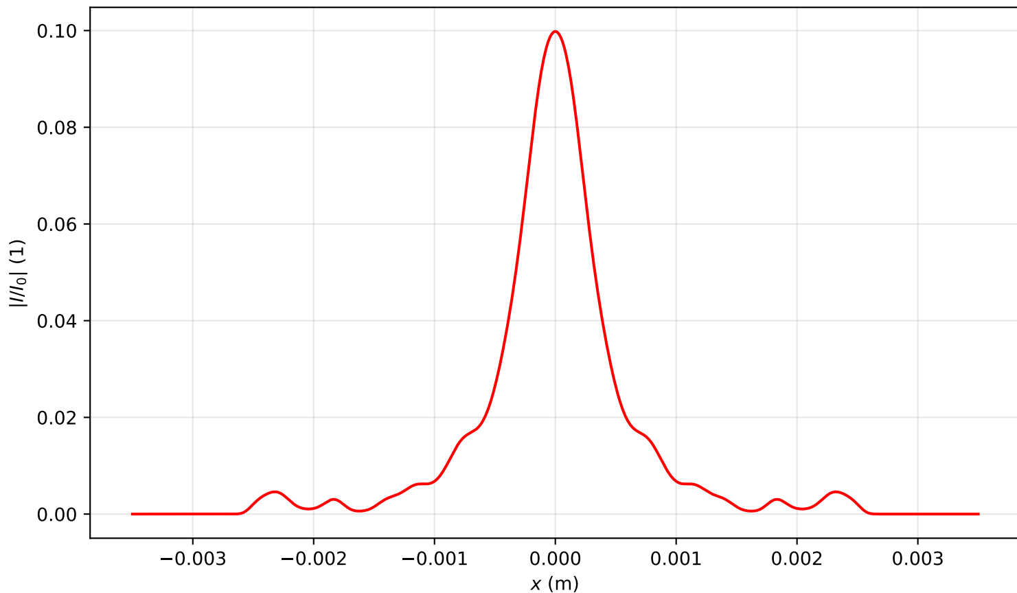
Intensity profile I(x, y = 0, z = 2.866)/I_0 , P_{in}=11.0P_{cr} , artificial time
