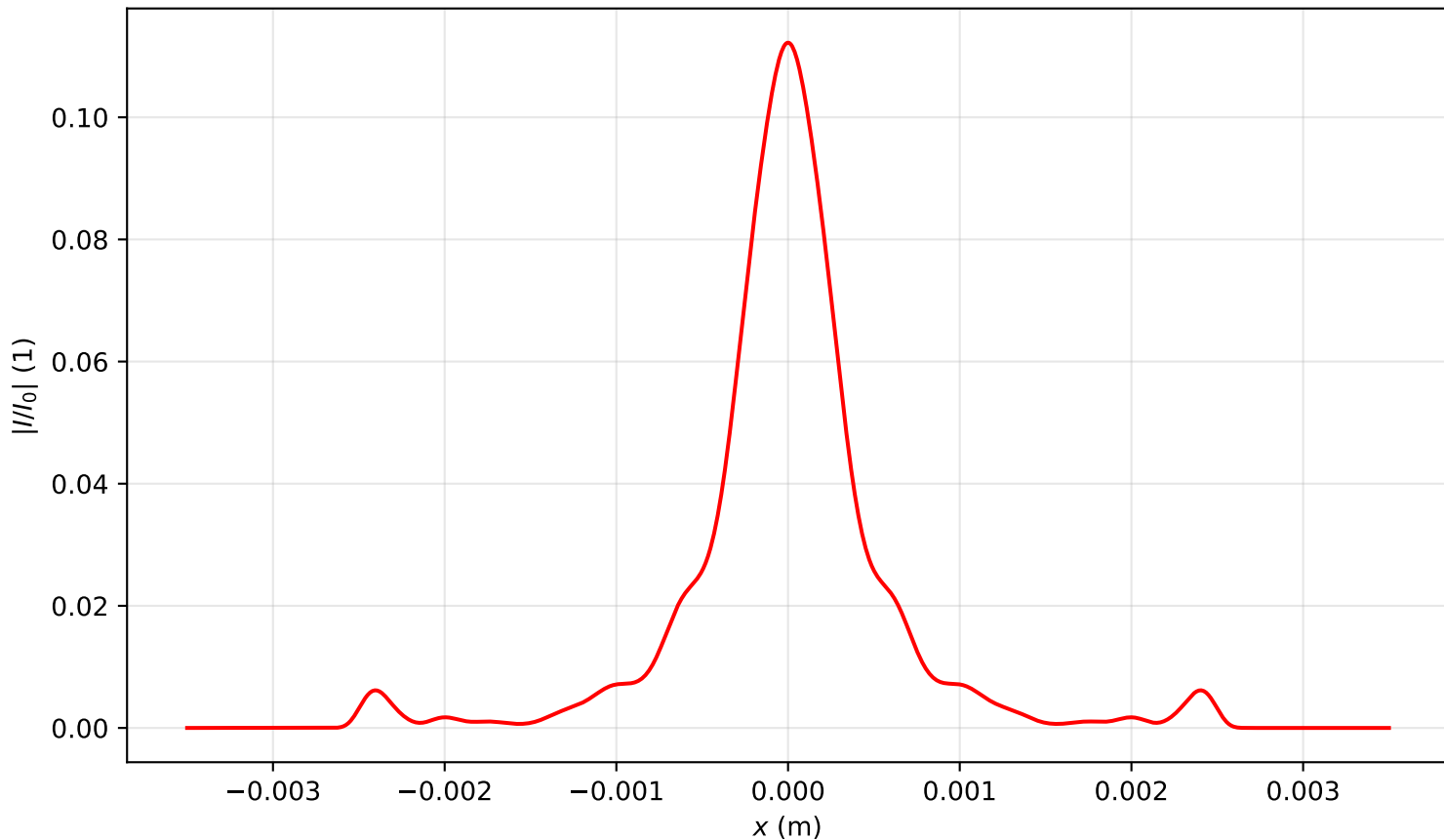
Intensity profile I(x, y = 0, z = 3.025)/I_0 , P_{in}=11.0P_{cr} , artificial time
