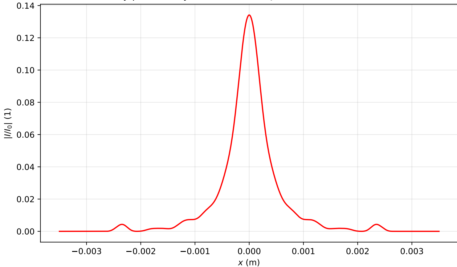
Intensity profile I(x, y = 0, z = 3.184)/I_0 , P_{in}=11.0P_{cr} , artificial time
