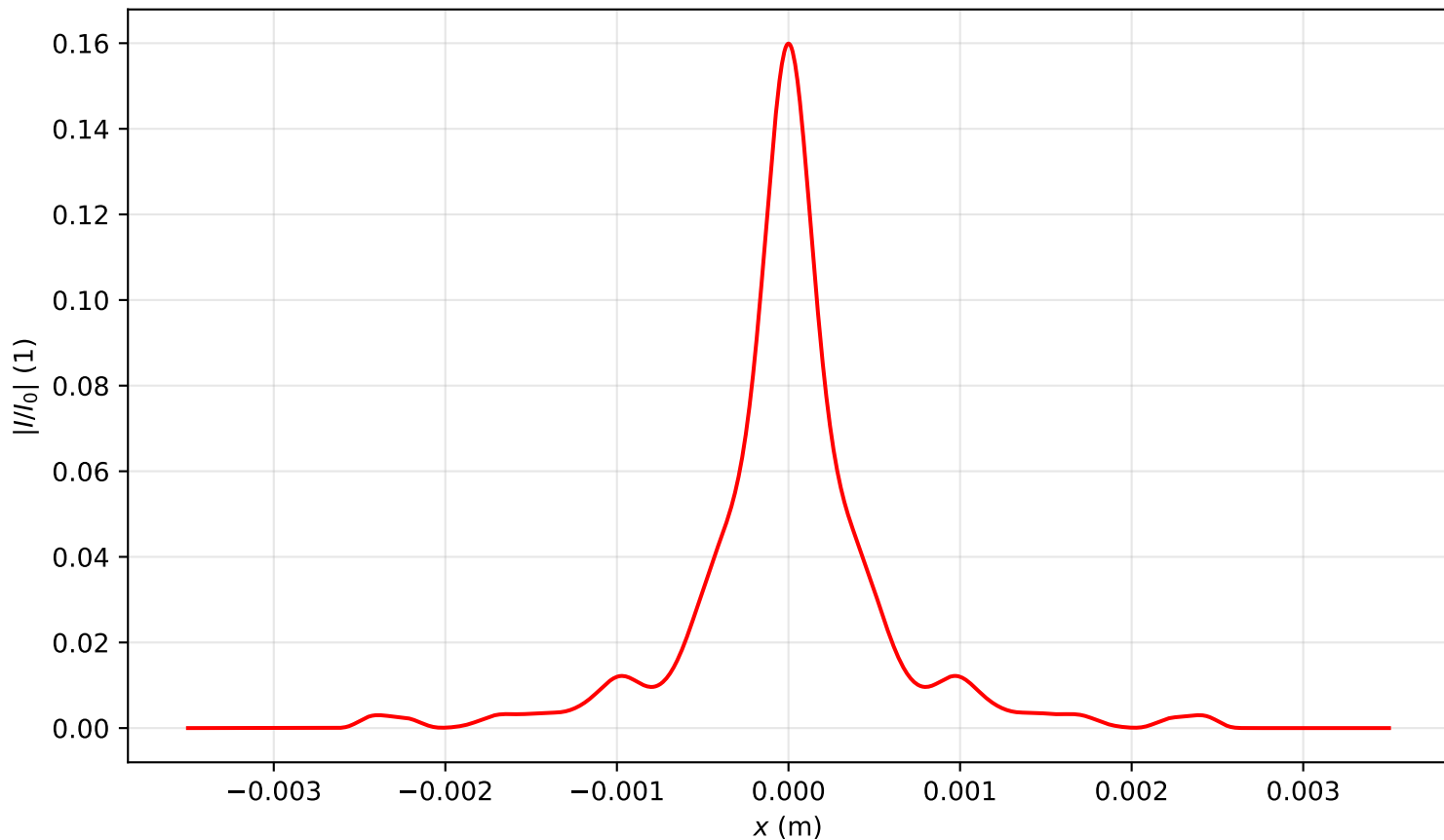
Intensity profile I(x, y = 0, z = 3.344)/I_0 , Pin=11.0Pcr, artificial time
