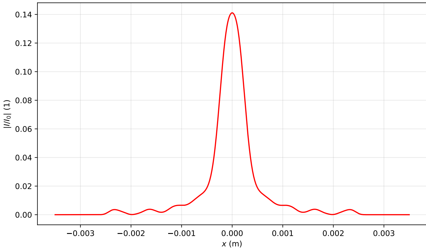
Intensity profile I(x, y = 0, z = 3.503)/I_0 , P_{in}=11.0\text{Pcr} , artificial time
