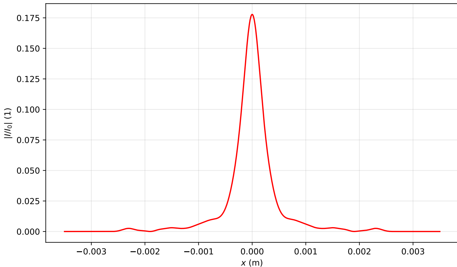
Intensity profile I(x, y = 0, z = 3.662)/I_0 , P_{in}=11.0\text{Pcr} , artificial time
