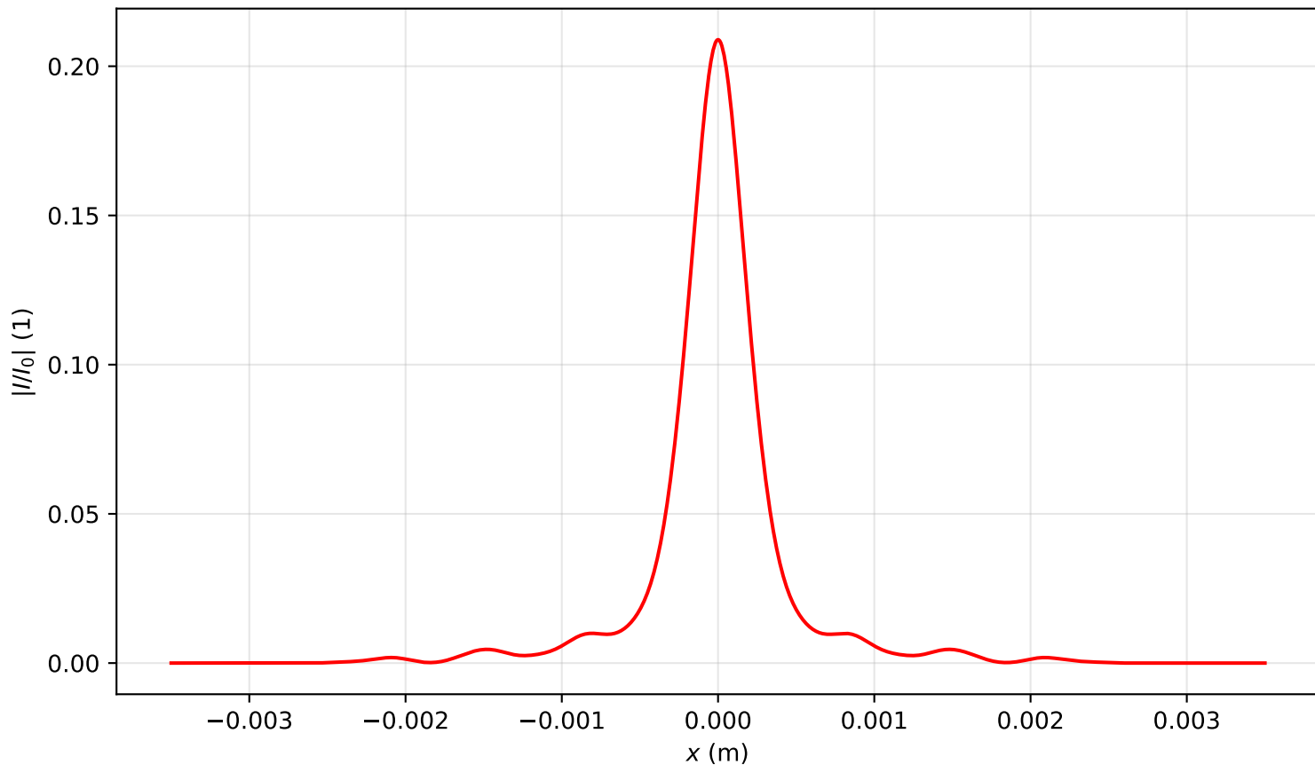
Intensity profile I(x, y = 0, z = 3.821)/I_0 , P_{in}=11.0P_{cr} , artificial time
