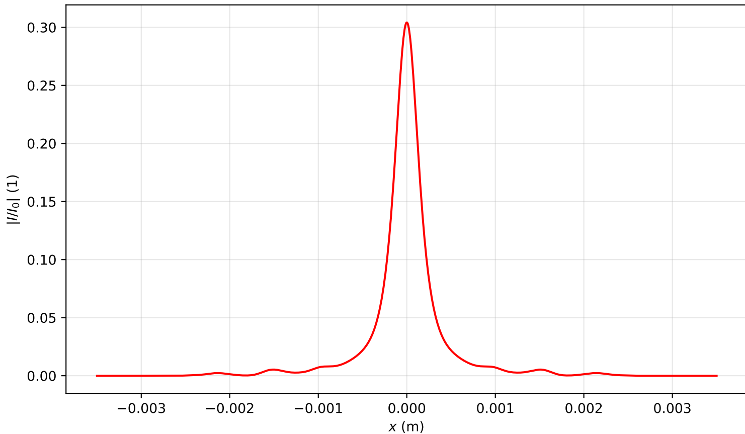
Intensity profile I(x, y = 0, z = 3.981)/I_0 , P_{in}=11.0P_{cr} , artificial time
