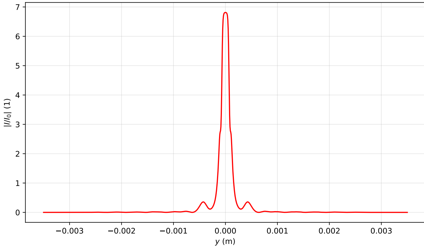
Intensity profile I(x=0, y, z=0.318)/I_0 , P_{in}=11.0P_{cr} , artificial time
