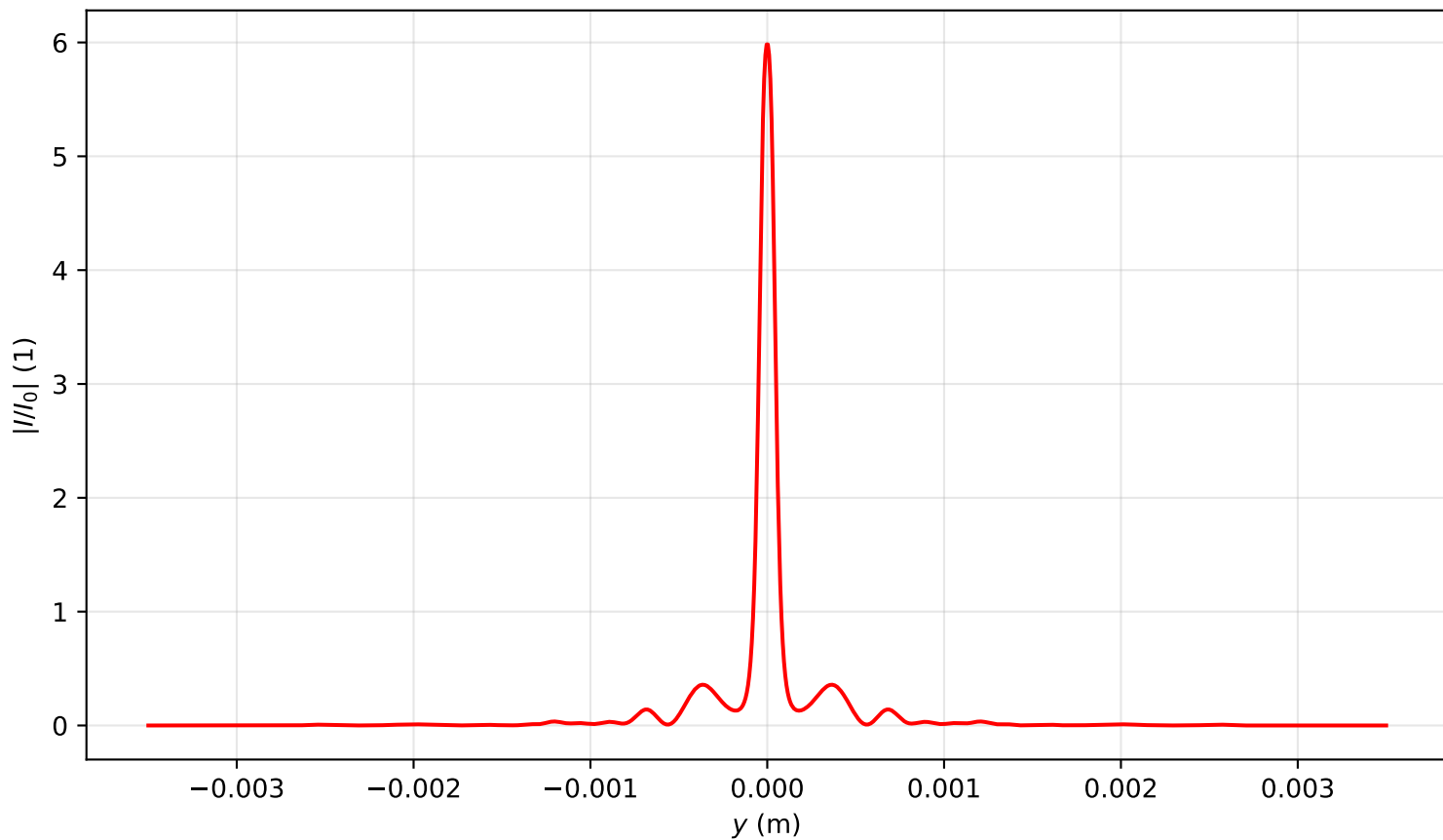
Intensity profile I(x=0, y, z=0.478)/I_0 , P_{in}=11.0P_{cr} , artificial time
