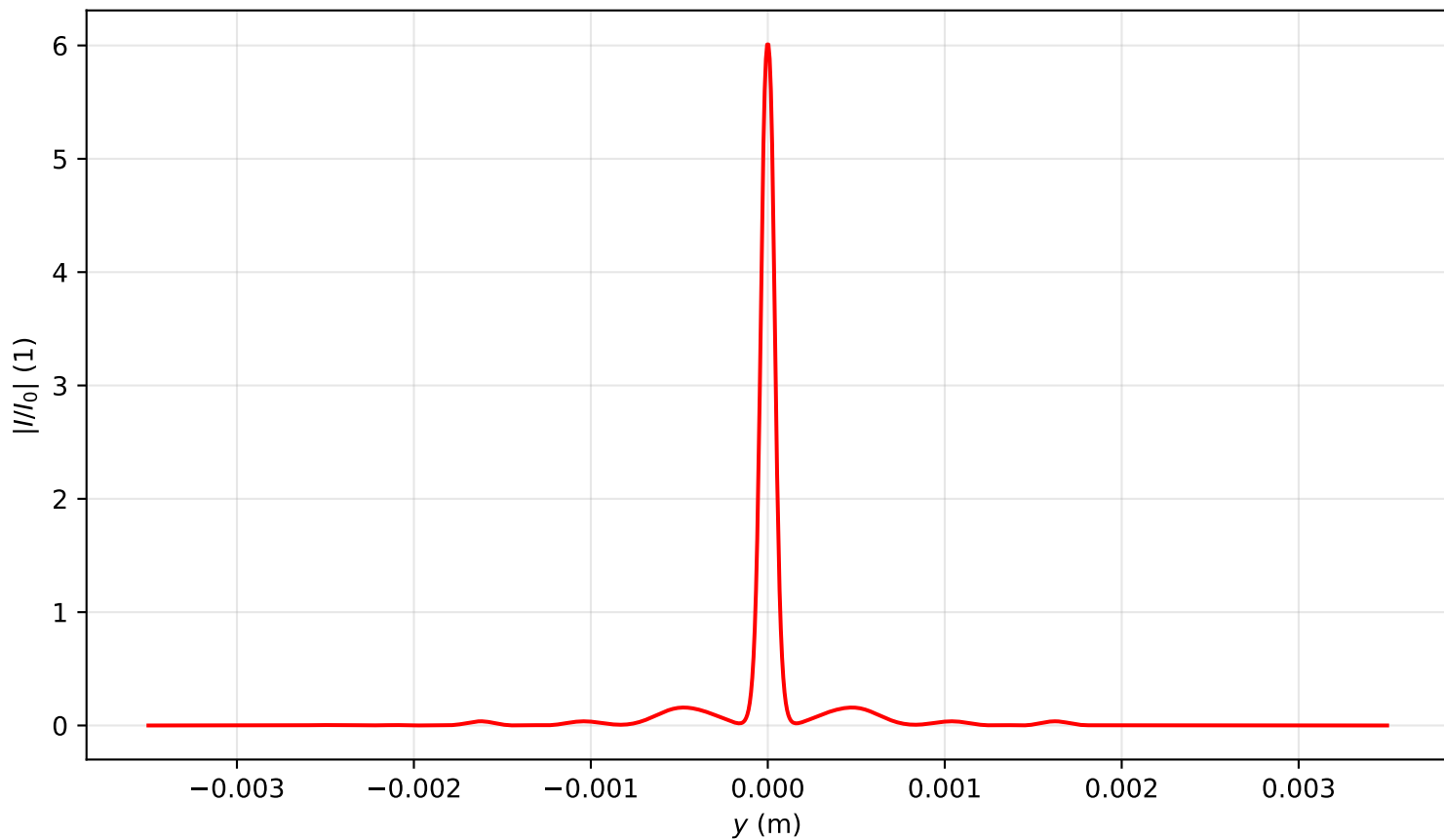
Intensity profile I(x=0, y, z=0.637)/I_0 , P_{in}=11.0P_{cr} , artificial time
