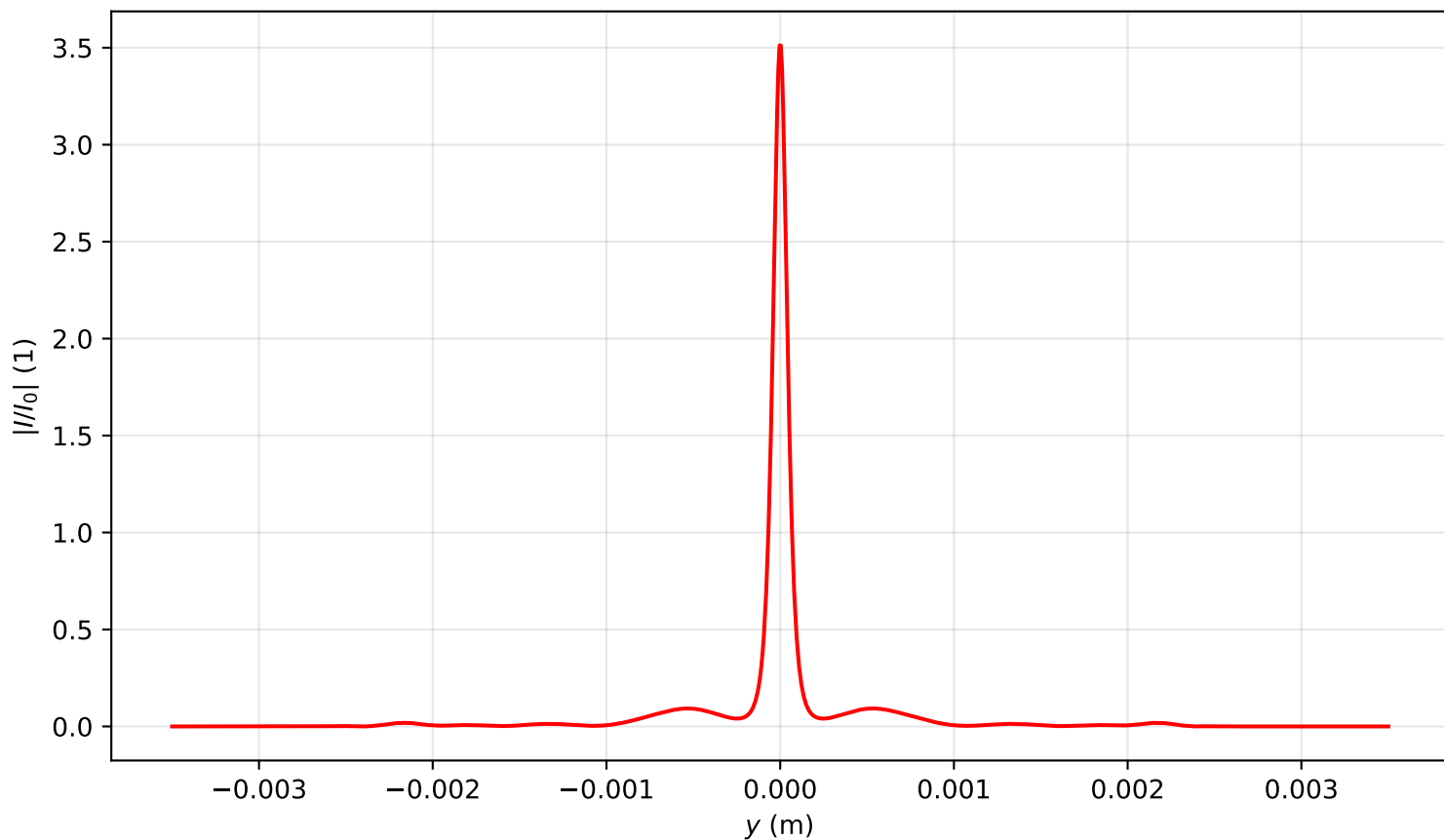
Intensity profile I(x=0, y, z=0.796)/I_0 , P_{in}=11.0P_{cr} , artificial time
