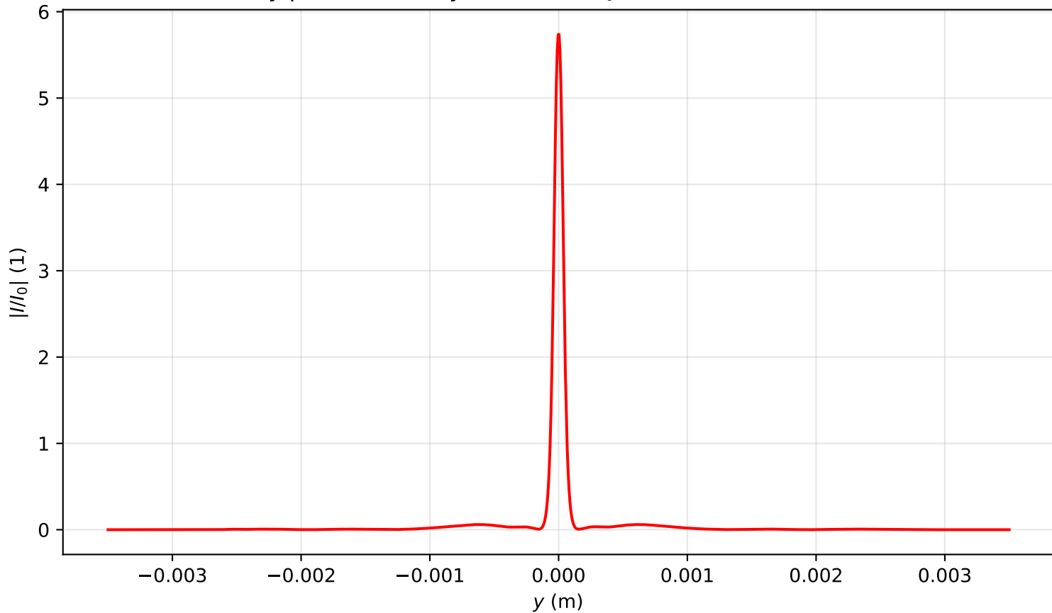
Intensity profile I(x=0, y, z=0.955)/I_0 , P_{in}=11.0P_{cr} , artificial time
