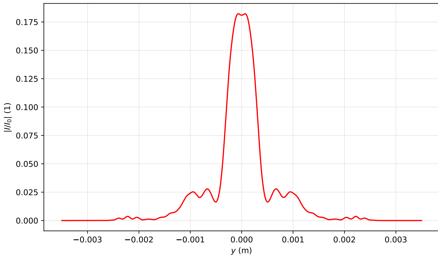
Intensity profile I(x=0, y, z=1.274)/I_0 , P_{in}=11.0\text{Pcr} , artificial time
