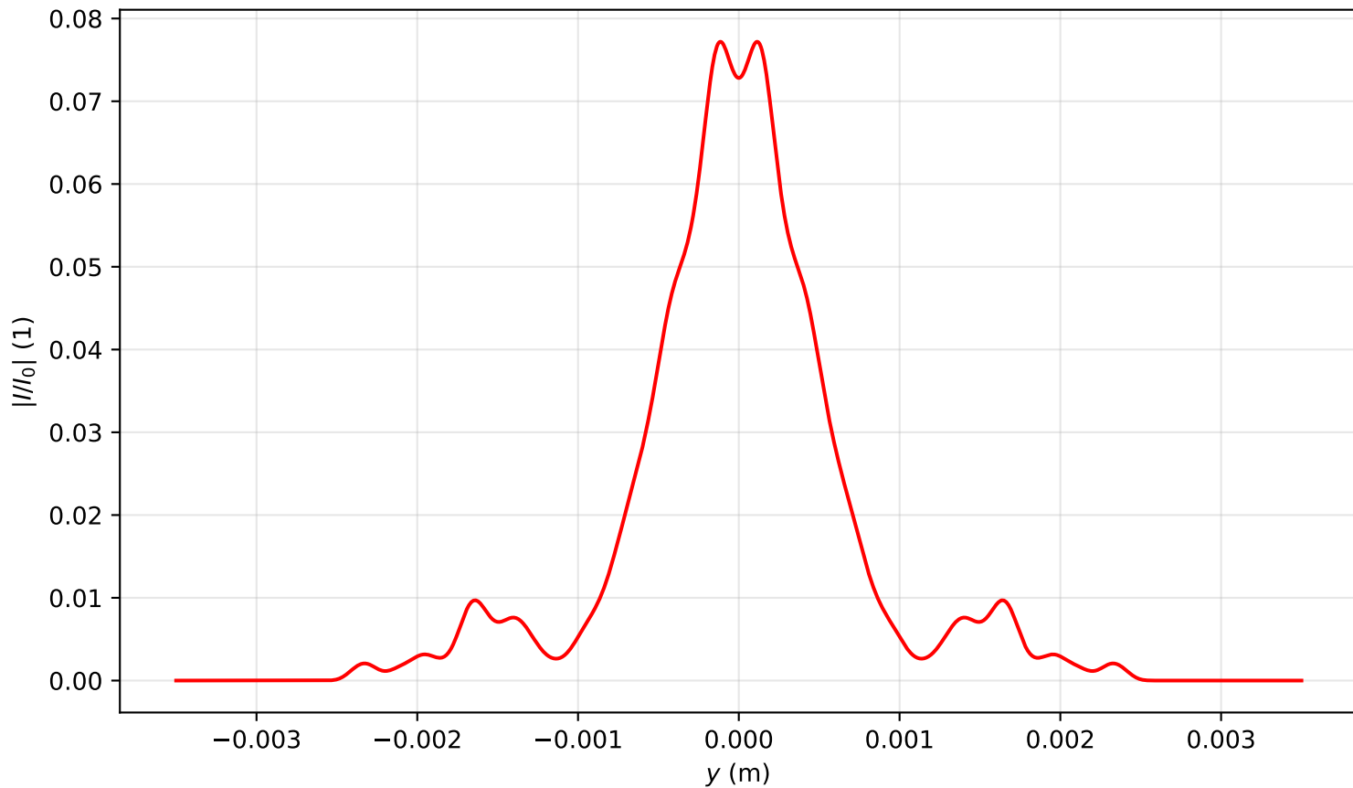
Intensity profile I(x=0, y, z=2.070)/I_0 , P_{in}=11.0P_{cr} , artificial time
